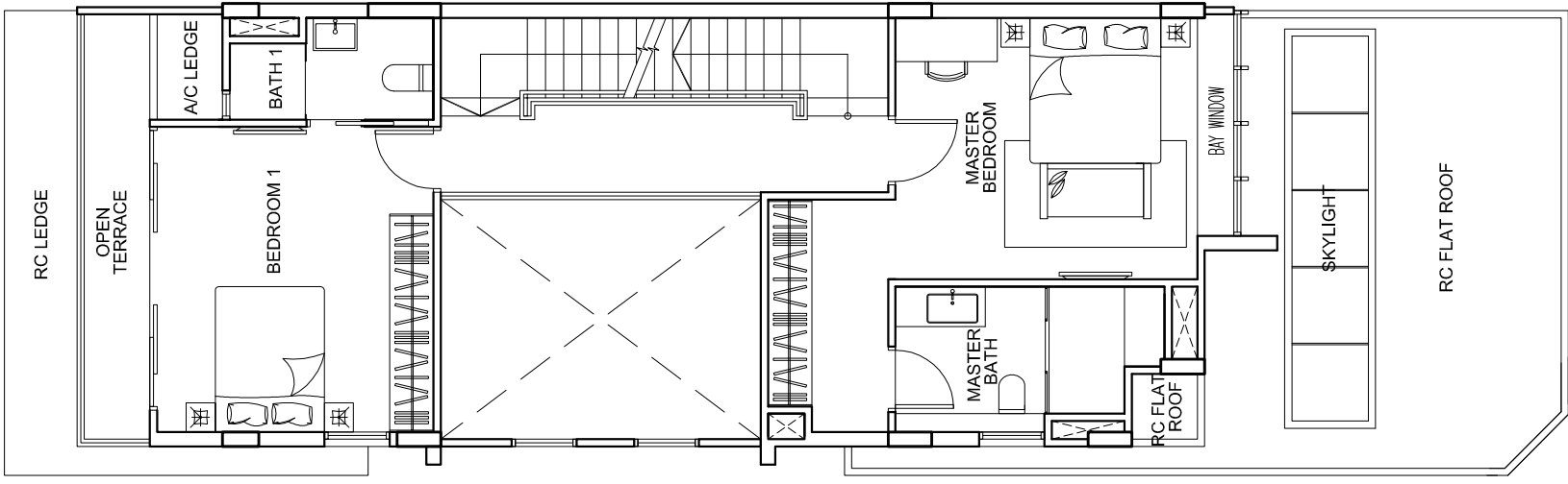
2nd Storey
